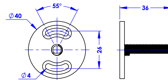
Platine de fixation. Fixing plate.
