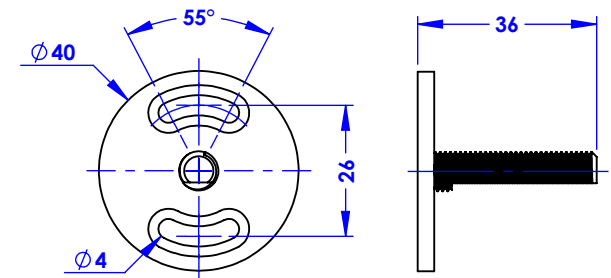
Platine de fixation. Fixing plate.
